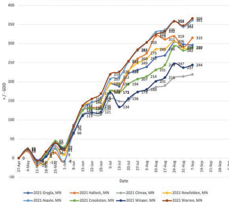
2021 Northwest Minnesota Departure From Normal
