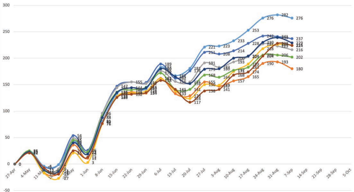
2021 Southwest Minnesota Departure From Normal
