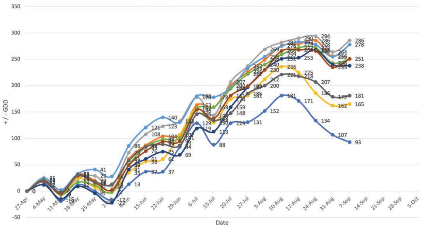
2021 Central and Northwest North Dakota
